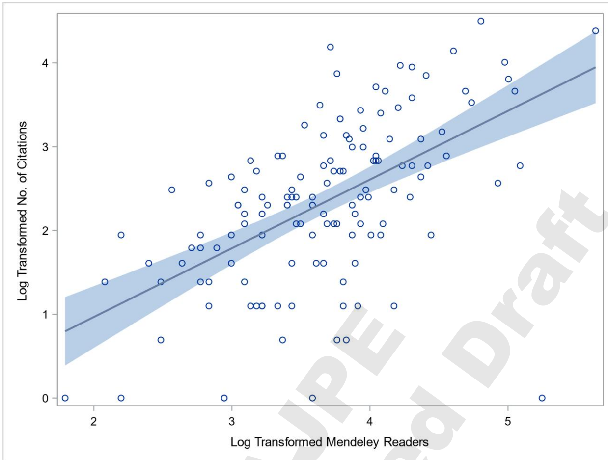
Figure 2. Relationship Between Log-Transformed 3-Year Number of Mendeley Readers and Log-Transformed 3-Year Number of Citations
